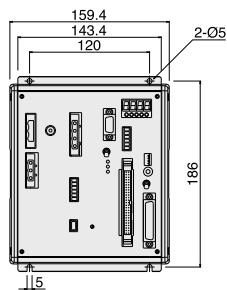
XSEL-K-1 (General-purpose, 1 axis)
