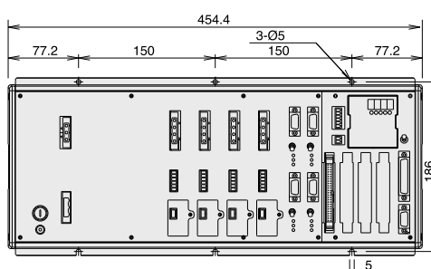
XSEL-K-4 (General-purpose, 4 axes)
