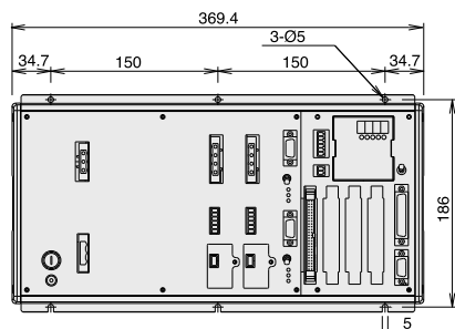
XSEL-K-2 (General-purpose, 2 axes)
