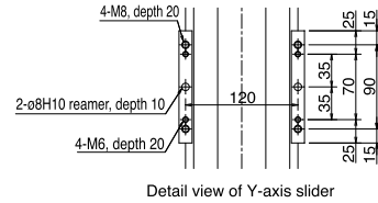
Detail view of Y-axis slider
