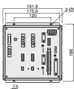
XSEL-K-3 (General-purpose, 3 axes)
